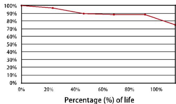
Lumen Maintenance (%)
